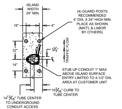
ISLAND DETAIL
